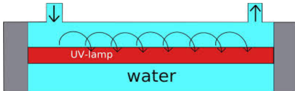
Structure & working principle of UV sterilizer
