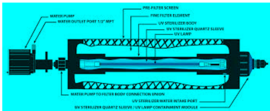
Structure & working principle of UV sterilizer
