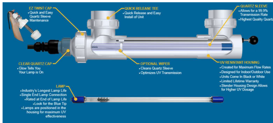
Structure & working principle of UV sterilizer
